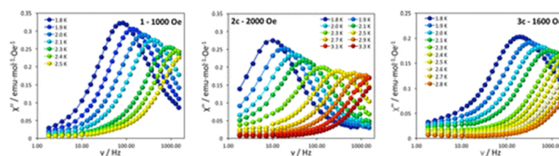
Fig. 15 Schematic representation of \text{Co}^{\text{II}} complexes 17 and 17a–17c (top) and field induced AC magnetic data for 17 , 17a and 17c at different temperatures (bottom), 91 adapted/reproduced from ref. 91 with permission from American Chemical Society, 91 copyright 2016.
