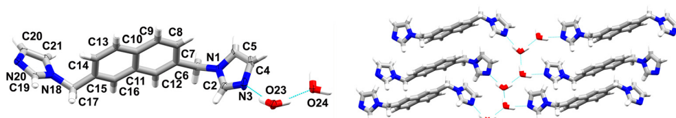
Fig. 4 On the left: molecular structure of 4 with atomic displacement plot shown at 50% probability; on the right: fragment of the 2D supramolecular layers, bridged by water molecules.
