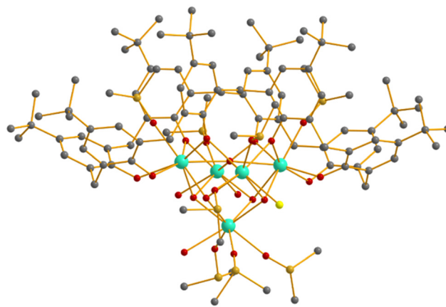
Fig. 17 The structure of the cation of compound 34 . Colour code: Tb = cyan, O = red, C = grey, S = dark yellow, Cl = yellow. H atoms omitted for clarity.
