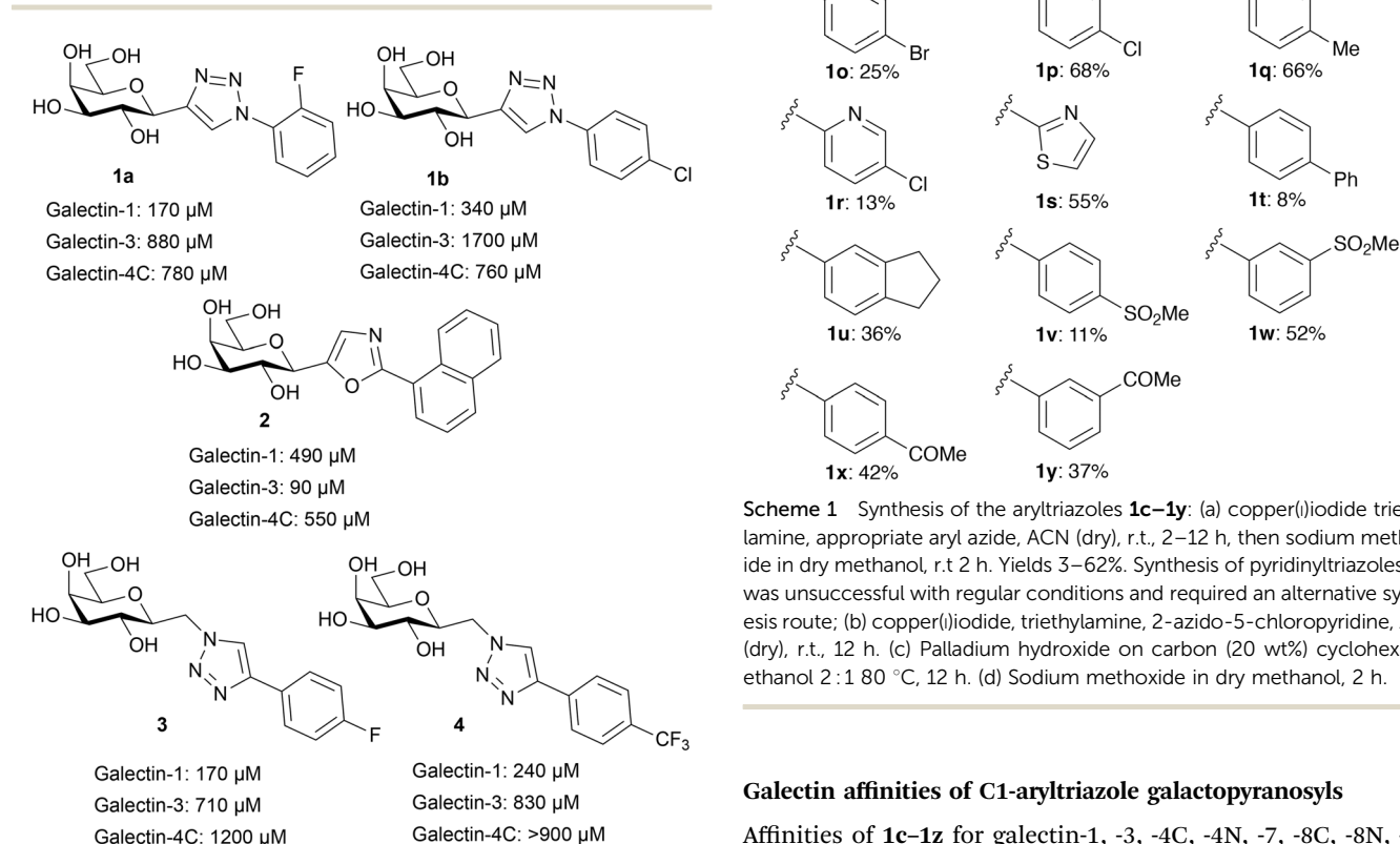
Chart 1 C1-Galactosyl galectin inhibitors with affinity and selectivity pattern. 54,55
