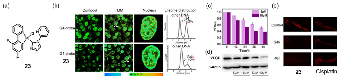
Fig. 5 (a) The chemical structures of the neutral complex 23 . (b) FLIM experiments of HeLa cells with 10 μM G-quadruplex-probe NBTE and 23 for 24 h. The descent of the G4-peak proved that 23 enters the nucleus and binds G4. (c) and (d) qRT-PCR and western blot results showed that 23 decreases VEGF mRNA transcriptions and VEGF protein levels in HeLa cells. (e) Complex 23 can effectively inhibit blood vessel growth in zebrafish, as red fluorescence changes show. 47 Copyright©2021, Wiley-VCH GmbH.
