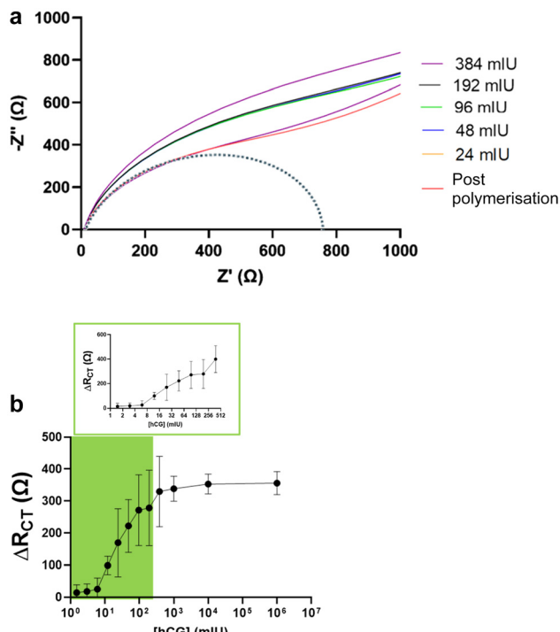
Fig. 4 (a) Nyquist plots of the E-layer-entrapped hCG nanoMIPs when exposed to a range of hCG concentrations. The derived R_{CT} is equivalent to the diameter of the pseudo semicircle extrapolated from the Nyquist plot at each concentration (an example semicircle given in the form of the dotted line). (b) Calibration curve of hCG levels vs. \Delta R_{CT} . Demonstration of the linear range for the E-layer-entrapped hCG nanoMIPs exposed to hCG in PBS between 1.5 and 384 mIU. As the hCG concentration increases, the \Delta R_{CT} value increases proportionately until saturation of the nanoMIP binding sites is reached. Error bars represent the standard deviations for averaged signals from 3 separate electrodes.
