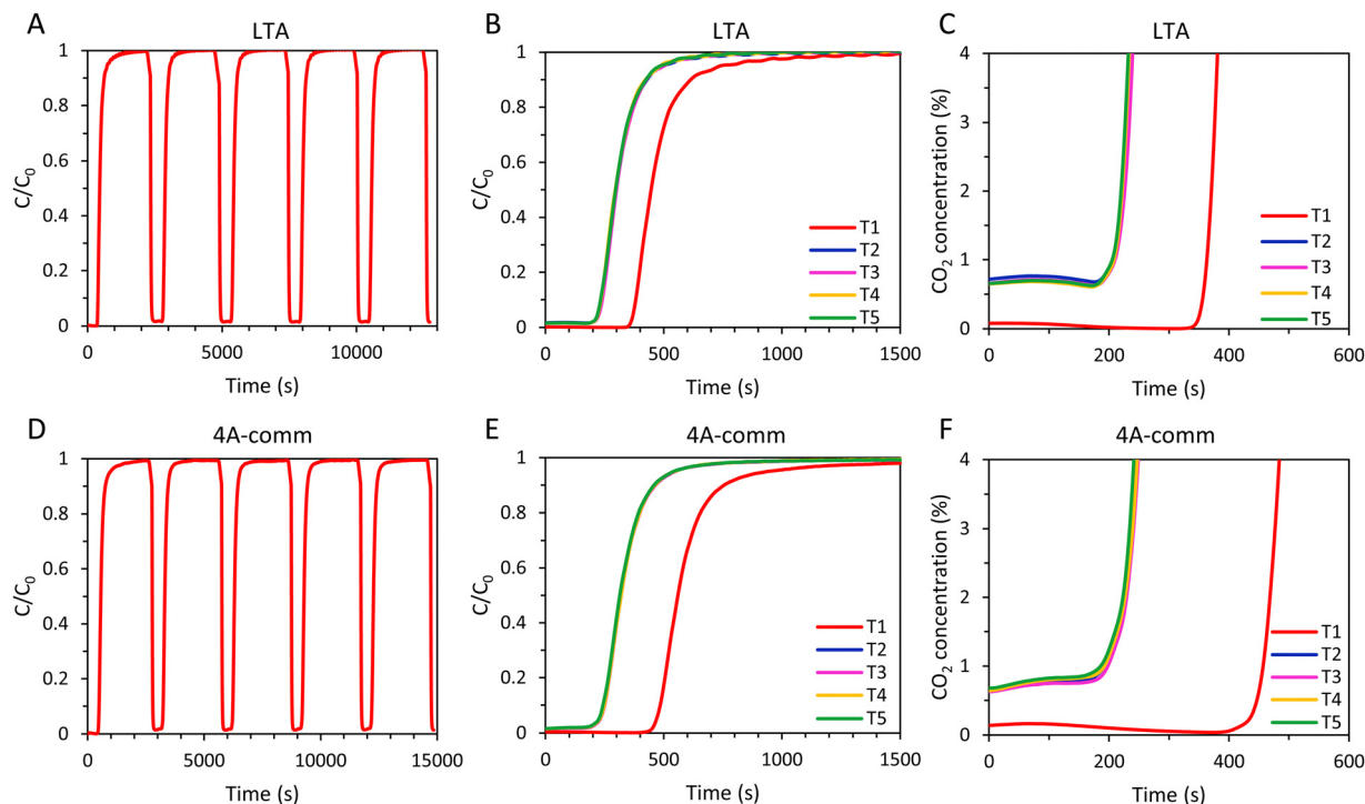
Fig. 6 (A) 5 consecutive adsorption–desorption cycles for LTA beads in a VPSA setup; (B) cyclic breakthrough curves of LTA beads (5 cycles); (C) cyclic breakthrough curves of LTA beads up to \text{CO}_2 concentration of 4% (5 cycles); (D) 5 consecutive adsorption–desorption cycles for 4A-comm beads in a VPSA setup; (E) cyclic breakthrough curves of 4A-comm beads (5 cycles); (F) cyclic breakthrough curves of 4A-comm beads up to \text{CO}_2 concentration of 4% (5 cycles). The adsorbents were regenerated in between cycles by evacuation at 20 mbar for 2 min, followed by flushing with \text{N}_2 for 139 s.
