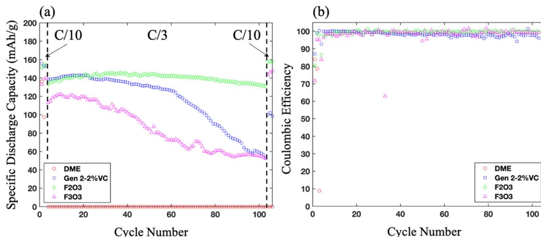
Fig. 5 (a) Discharge capacity and (b) coulombic efficiency profiles of as a function of cycle number for cells containing 1 M LiTFSI DME/ \text{F}_2\text{O}_3 / \text{F}_3\text{O}_3 electrolytes and 1 M LiPF 6 in EC/EMC (3/7) and 2% vinylene carbonate.
