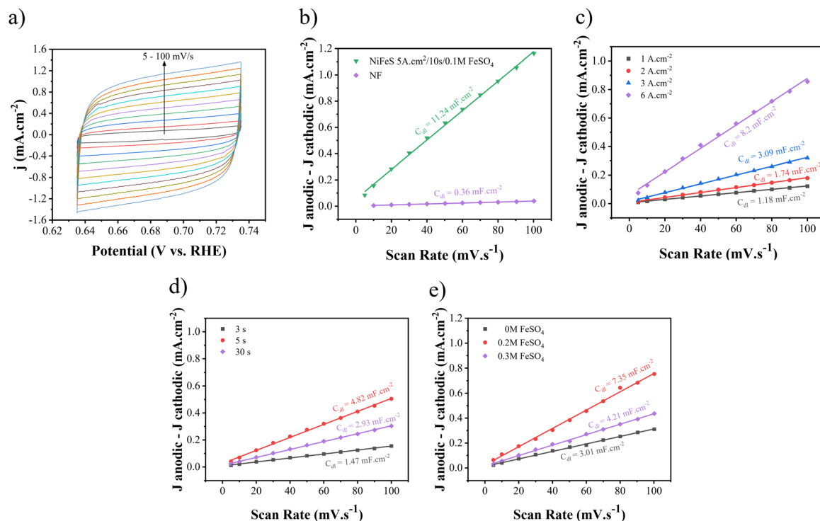
Fig. 9 (a) CV curves with different scan rates (5–100 mV s -1 ) and C dl plots for (b) optimum Ni–Fe–S and NF and Ni–Fe–S synthesized at (c) different electrodeposition current densities, (d) different duration times, and (e) different concentrations of FeSO 4 .
