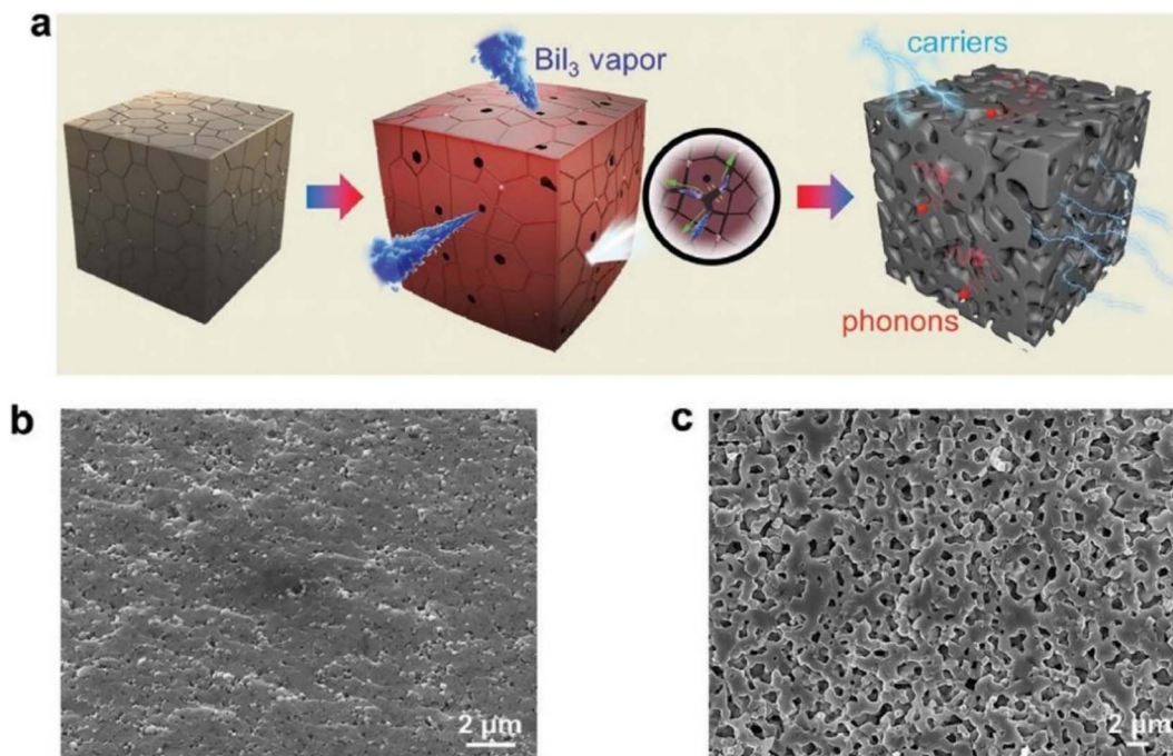
Fig. 21 (a) 3D pictorial representation of porous network generation during the BiI 3 sublimation. SEM images of the fracture surface: (b) AD 0 vol% and (c) AP 0.7 vol%. Reproduce from ref. 65.
