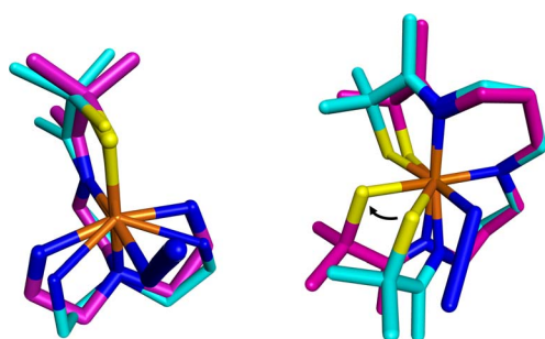
Fig. 12 Visualization of experimentally obtained structural changes that occur upon oxidation and binding of a sixth ligand, azide. Left: [Fe II (S Me2 N 4 (tren))] + ( 4 , cyan) 36 to [Fe III (S Me2 N 4 (tren))N 3 ] (magenta). 37 Right: [Fe II (S 2 Me2 N 3 (Pr,Pr))] ( 1 , cyan) 22 and [Fe III (S 2 Me2 N 3 (Pr,Pr))(N 3 )] (magenta). 31 Depiction utilized previously reported crystallographically determined structures.
