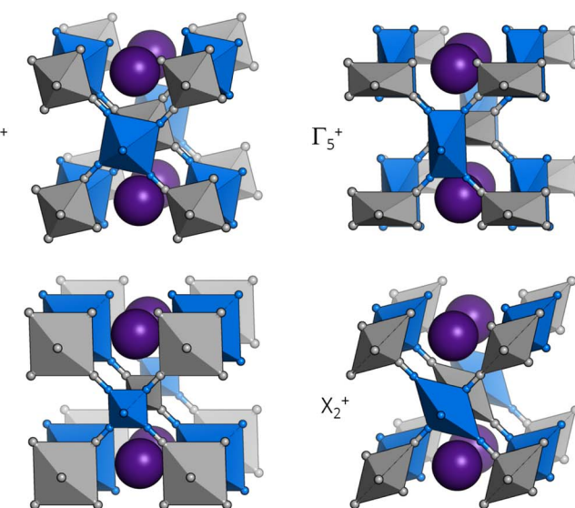
Fig. 3 The left panel shows the pressure evolution of the tilt angles of RbCuCo, with \angle\text{CuCoC} in black and \angle\text{CoCuN} in orange, and the CuN bond lengths of RbCuCo as a function of pressure. The right panel visualises the distortion modes (with exaggerated amplitudes) potentially driving the phase transition in RbCuCo.
