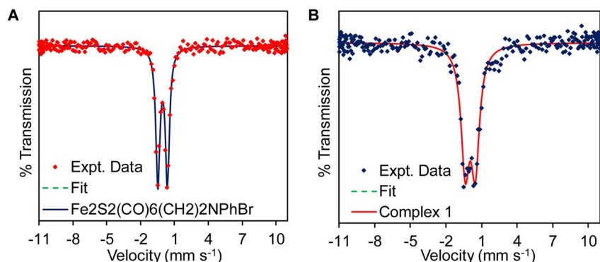
Fig. 2 Mössbauer spectra of the (A) precursor complex and (B) complex 1 recorded at 90 K.
