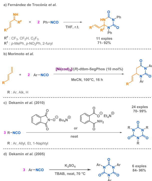
Scheme 5 Synthesis of uracil and aza-uracil derivatives via pseudo-MCR methodologies.
