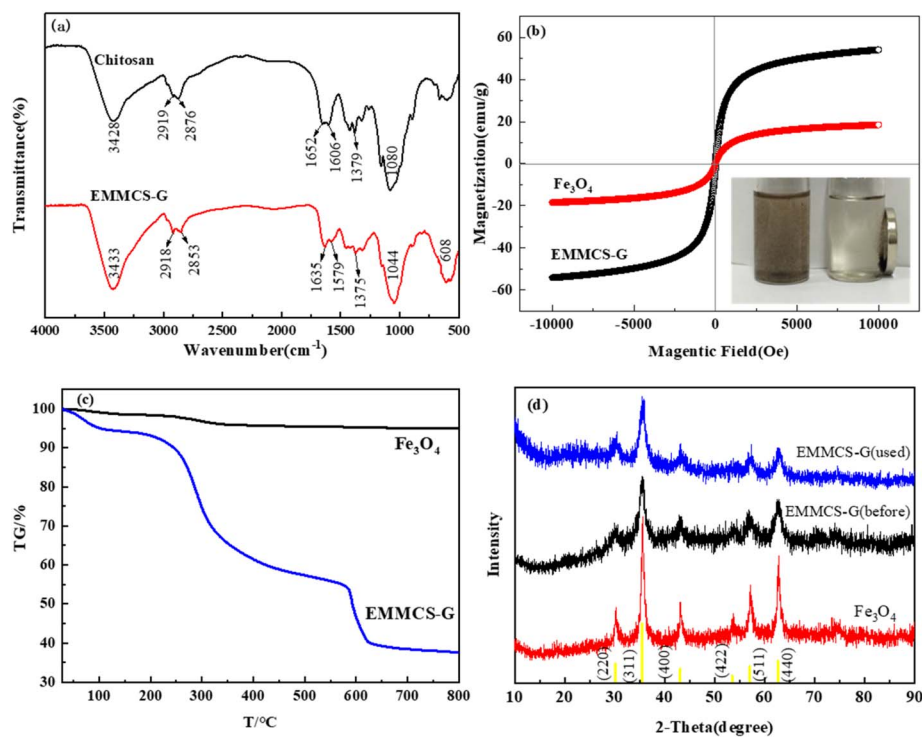
Fig. 2 (a) FTIR spectra of chitosan and EMMCS-G. (b) Magnetic hysteresis loops of \text{Fe}_3\text{O}_4 and EMMCS-G. (c) TGA curves of \text{Fe}_3\text{O}_4 and EMMCS-G. (d) XRD patterns of \text{Fe}_3\text{O}_4 and EMMCS-G before and after reaction in EMMCS-G/PS system.
