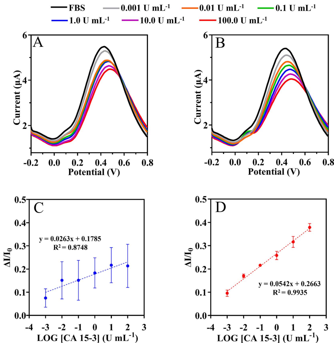
Fig. 8 SWV measurements of NIPs (A) and MIPs (B) based biosensor and the corresponding calibration curves (C) and (D) respectively, in 5 mmol L -1 [Fe(CN) 6 ] 3- and 5 mmol L -1 [Fe(CN) 6 ] 4- by increasing CA 15-3 protein in the fetal bovine serum.
