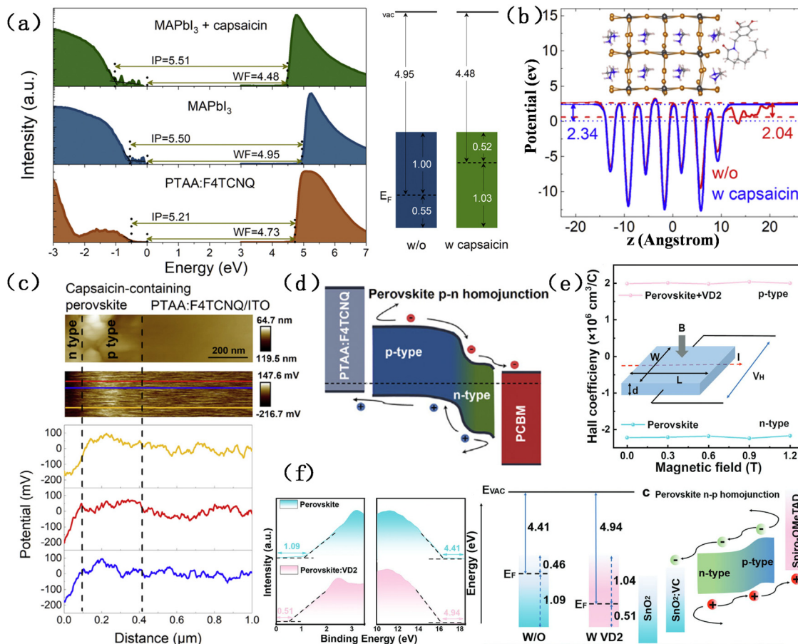
Fig. 12 (a) UPS spectra of the secondary electron cutoff region and valence band region. (b) Calculated electrostatic potential and Fermi level of the perovskite surface with and without capsaisin. (c) Cross-sectional AFM topographies, corresponding KPFM images, and potential profiles under zero-voltage bias. (d) Energy level alignment schematics of the PSC comprising capsaisin. 28 Copyright 2021, Elsevier. (e) Hall effect measurement of perovskite films. The inset shows the Hall effect measurement setup. (f) UPS spectra and energy level alignment schematics. 86 Copyright 2023, Wiley.
