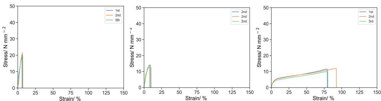
Fig. 2 Stress strain curve for 10E 15 -1 (left), 10E 15 -2 (middle) and 10E 15 -3 (right) under uniaxial tension at 50 \text{ mm s}^{-1} .
