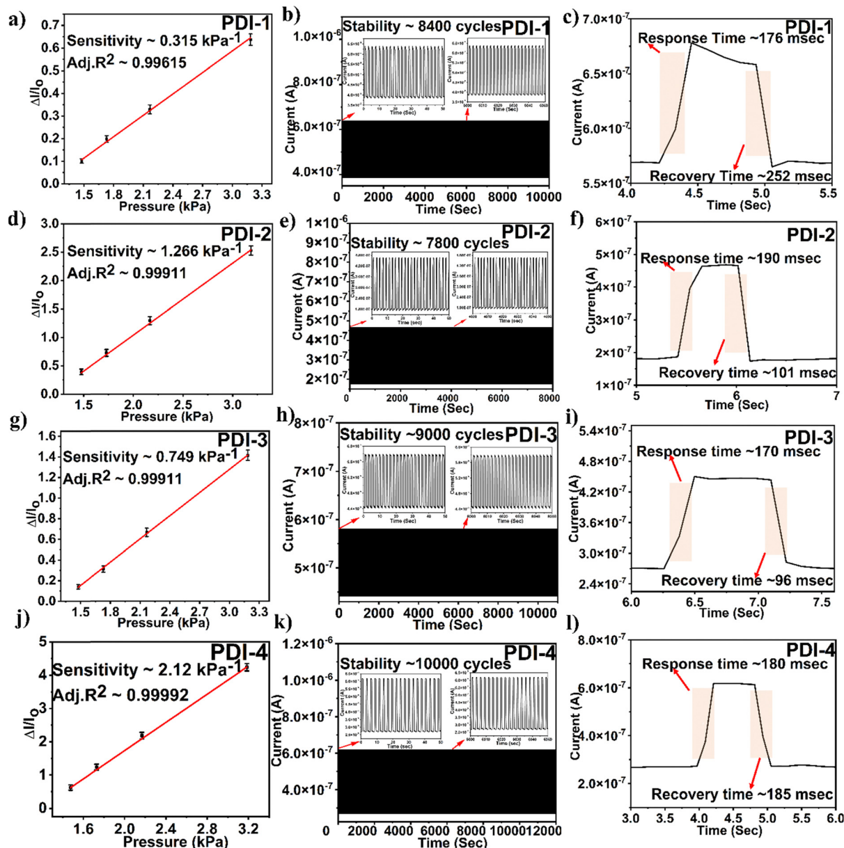
Fig. 6 (a), (d), (g) and (j) Normalized current vs. applied pressure to attain sensitivity, (b), (e), (h) and (k) endurances of the fabricated sensors, and (c), (f), (i) and (l) response and recovery times for fabricated PDI-based pressure sensors.
