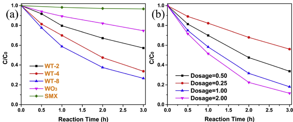
Fig. 11 (a) SMX degradation under visible-light irradiation by WO 3 , WT-2, WT-4 and WT-8. Conditions: catalyst: 0.50 g L -1 , SM: 10 mg L -1 . (b) SMX degradation by WT-4 at different catalyst dosage (0.25, 0.50, 1.00 and 2.00 g L -1 ). Conditions: SMX: 10 mg L -1 . (c) Schematic illustration of the proposed mechanism for the enhanced degradation of SMX by WO 3 -CNT composites under visible-light irradiation. Reproduced from ref. 261 with permission from Elsevier (2018).
