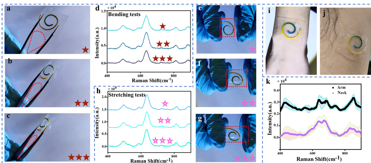
Fig. 4 Sweat platform flexibility, stretchability, and stability. Photographs of the sweat platform: (a) slightly twisted, (b) overly twisted, (c) fully twisted; (d) SERS spectra of UA collected at different degrees of bending. Photographs of the sweat platform (e) under 10% stretch, (f) under 20% stretch, (g), and under 30% stretch; (h) SERS spectra of UA collected at different degrees of stretch. Photographs of the sweat platform conformally laminated on the human subject: (i) the arm and (j) the neck. (k) SERS spectrum of the sweat collected from the arm and neck.
