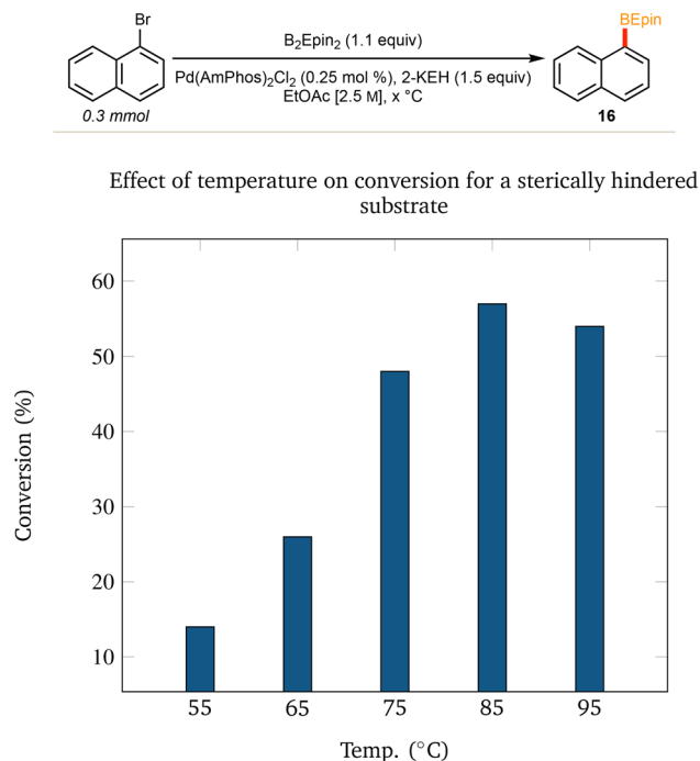
Fig. 3 Temperature study Effect of temperature on conversion for a sterically hindered substrate ( 1 H NMR conversions).
