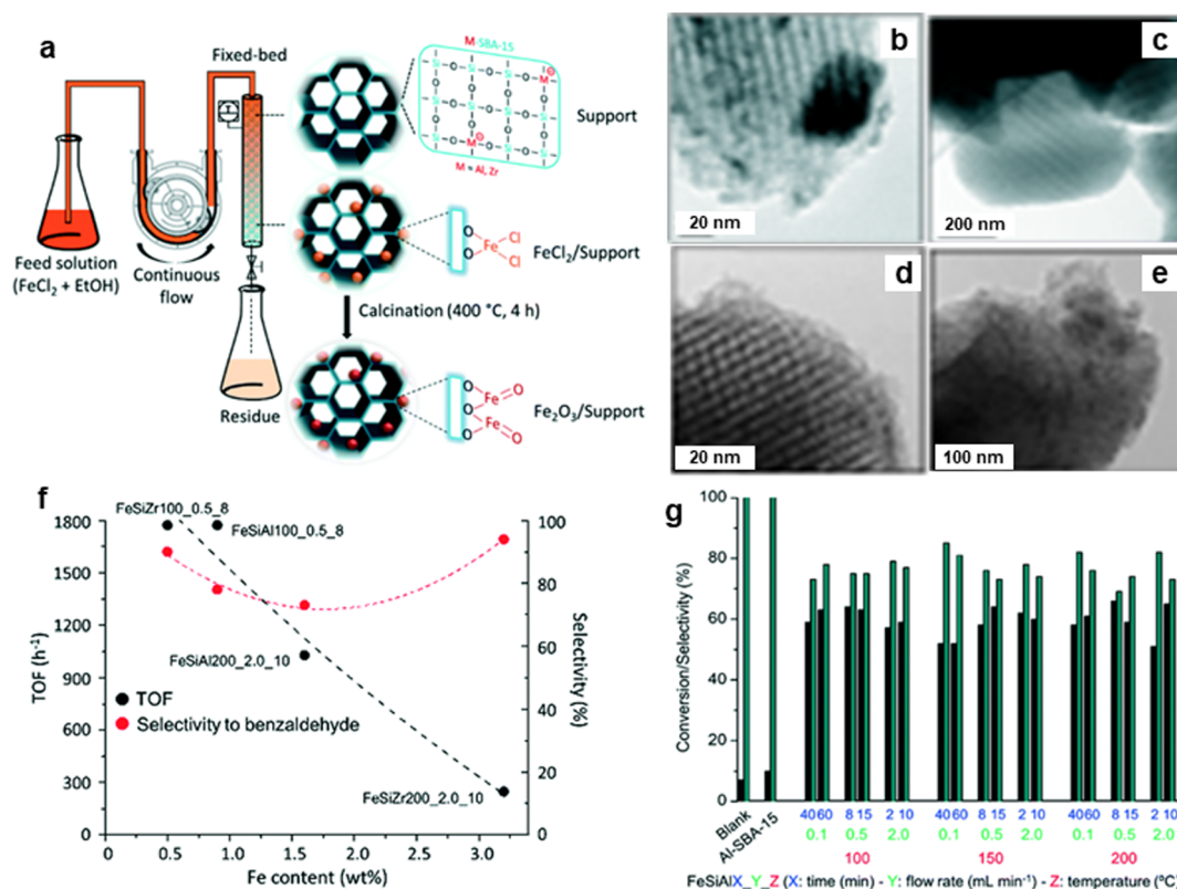
Fig. 30 (a) Schematic for continuous flow synthesis of \text{Fe}_2\text{O}_3 NPs; (b–e) TEM images of \text{FeAlSi150}_0.1_40 , \text{FeZrSi150}_0.1_40 , \text{FeSiAl200}_0.1_40 and \text{FeZrSi200}_0.1_40 catalysts respectively, (f) Effect of Fe loading on TOF and selectivity, and (g) Performance of catalysts on conversion and selectivity. Reproduced with permission from ref. 213 Copyright 2018, The Royal Society of Chemistry.
