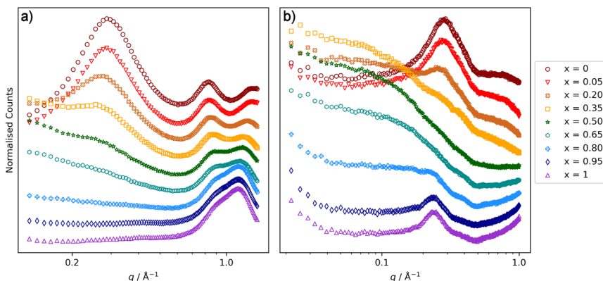
Fig. 5 (a) SAXS data and (b) SANS data collected for [\text{C}_{10}\text{MIM}]_{1-x}[\text{C}_{10}\text{MIM-F}_{17}]_x[\text{Tf}_2\text{N}] mixtures at 60 \text{ }^\circ\text{C} . Data for each composition are shifted along the y-axis for clarity. Note the different scales used for the x-axes.
