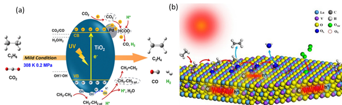
Fig. 17 (a) Schematic representation of (a) photocatalytic oxidative dehydrogenation of C_2H_6 with \text{CO}_2 over \text{Pd/TiO}_2 ; Reproduced with permission. 108 Copyright 2018, American Chemical Society and (b) photocatalytic C_2H_6 dehydrogenation over \text{LaVO}_4\text{-O}_v ; reproduced with permission. 110 Copyright 2024, Elsevier.
