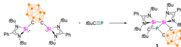
Scheme 4 Reaction of [LSiBSiL] and t BuC≡P.
