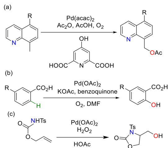
Scheme 1 Pd-catalyzed C–H functionalization reactions with \text{O}_2 or \text{H}_2\text{O}_2 as oxidants.
