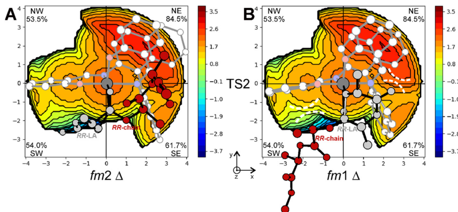
Fig. 3 Steric maps obtained by the % V_{Bur} analysis explaining the energetic preference for fm2 (A) vs. fm1 (B) wrapping modes in the ring opening step (TS2) of RR -LA polymerization promoted by the (R) -1 system. The main steric interactions are reported with dashed lines.
