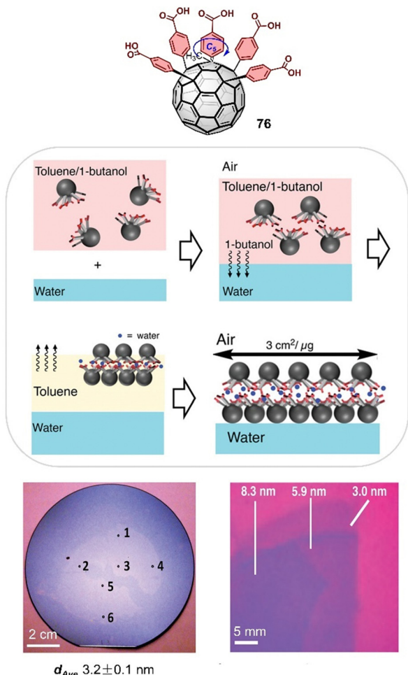
Fig. 30 Structure of pseudo- C_5 symmetric fullerene amphiphile 76 , assembly of 2D film, the 2D film on 160.6 \pm 0.1 nm thick SiO 2 /Si wafer ( \phi = 10.2 cm) (the thickness of six points were calculated by interference fringe shifts from visible-light reflection spectra), and sequential lamination of film on 288.8 nm thick SiO 2 /Si wafer to form single, double, and triple films. Adapted from ref. 461 with permission from Wiley-VCH, copyright 2022.
