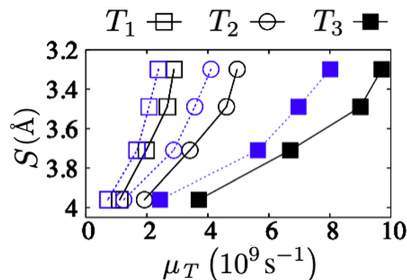
Fig. 8 Electron transfer rates \mu_T in \text{Ni}_3(\text{HITP})_2 as a function of the inter-layer spacing S at different temperatures of T_1 = 290 K, T_2 = 296 K, and T_3 = 298 K. Black profiles correspond to the eclipsed packing whereas the blue profiles refer to the slipped-parallel packing. All parameters and their corresponding units are reported in the ESI,† Tables S2–S4.
