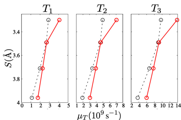
Fig. 9 Comparison between electron (black) and hole (red) transfer rates in the \text{Ni}_3(\text{HITP})_2 nanosheet as a function of the inter-layer spacing S at different temperatures of T_1 = 290 K, T_2 = 296 K, and T_3 = 298 K. All parameters and their corresponding units are reported in the ESI,† Tables S2–S4.
