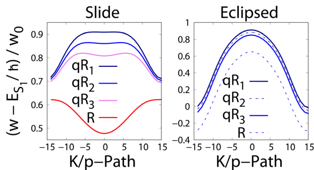
Fig. 5 Momentum( k )-exciton ( E ) dispersion profiles as a function of the energy difference E_{T-S_1} . Left (right) panel corresponds to the slide (eclipsed) configuration between consecutive monomers. The full set of parameters is reported in the ESI,† Table S2.
