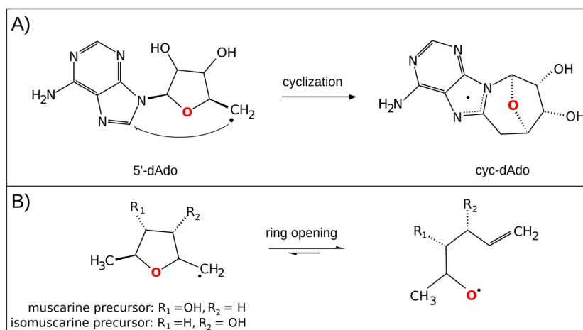
Fig. 1 (A) In the cyclization decay mechanism, the 5'\text{-dAdo}^{\bullet} radical undergoes intramolecular radical addition leading to a stable cyclic structure. 20 (B) The ring-opening decay mechanism was observed for the radicals similar to 5'\text{-dAdo}^{\bullet} . 21
