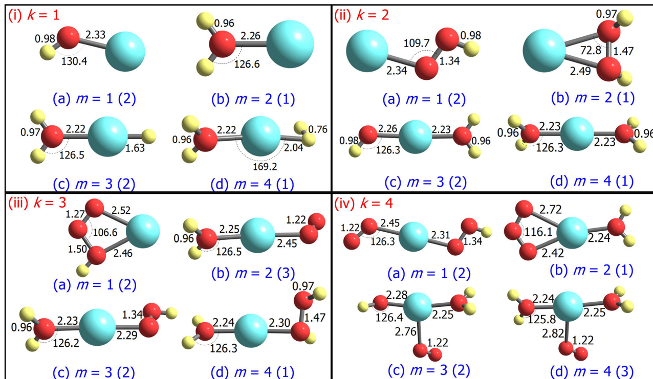
Fig. 1 Ground state structures of \text{AgO}_k\text{H}_m^+ , where k, m = 1-4 , optimized at the CCSD level. Bond lengths and angles are given in Å and degrees, respectively. The spin multiplicity (2S+1) of the \text{AgO}_k\text{H}_m^+ clusters is provided in the parentheses.
