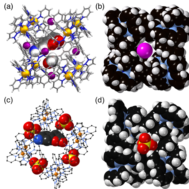
Fig. 10 Results of crystalline sponge experiments using \mathbf{H} as the host in which a cavity-bound guest (4-methyl-7-aminocoumarin, MAC) and surface bound guest anions are taken up to different sites in the same experiment. In (a) and (b) the surface-bound anion is iodide; in (c) and (d) it is sulfate. The wireframe cage views in (a) and (c) emphasise the location of the MAC guest; the space-filling views in (b) and (d) emphasise the locations of the anions in the surface portals.
