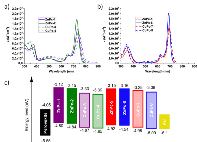
Fig. 4 UV-vis absorption spectra of MPcs in solution, (a) symmetric MPcs, (b) asymmetric MPcs, and (c) energy level diagram for the MPcs.
