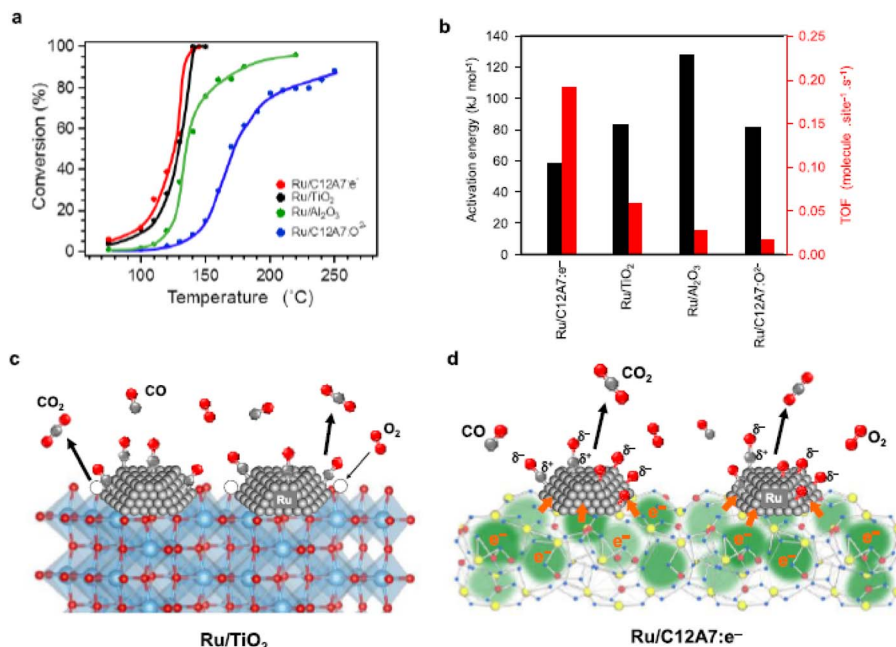
Fig. 11 (a) Catalytic activity for CO oxidation over various supported Ru catalysts. (b) TOFs and activation energies of the tested Ru catalysts. (c and d) Reaction pathways for CO oxidation on (c) Ru/TiO 2 and (d) Ru/C12A7:e - . Copyright 2015, American Chemical Society.
