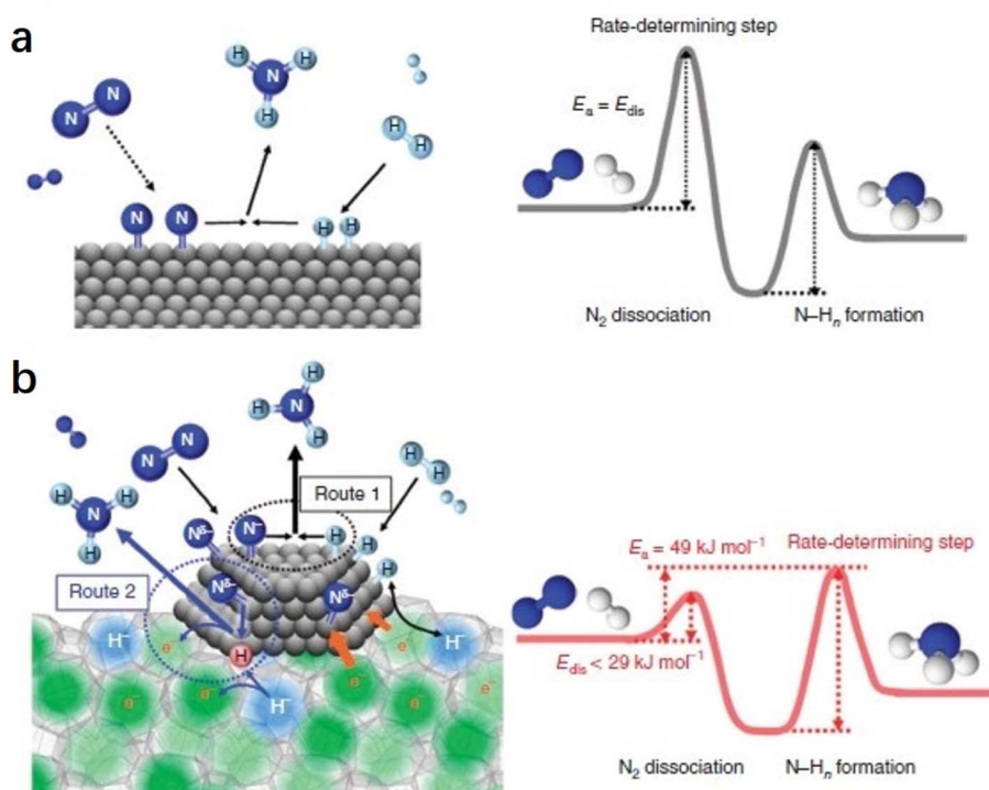
Fig. 7 Reaction mechanism and energy diagram for \text{NH}_3 synthesis on (a) conventional catalyst and (b) \text{Ru}/\text{C12A7}:\text{e}^- catalyst. Copyright 2015, Springer Nature.
