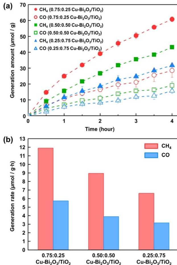
Fig. 18 (a) Amount of \text{CH}_4 and CO generated upon using 0.75 : 0.25, 0.50 : 0.50, and 0.25 : 0.75 Cu-Bi 2 O 3 / \text{TiO}_2 photocatalysts. (b) Rates of \text{CH}_4 and CO generation in the first 4 h of irradiation. Reproduced with permission from ref. 217, Copyright 2016 European Chemical Societies Publishing.
