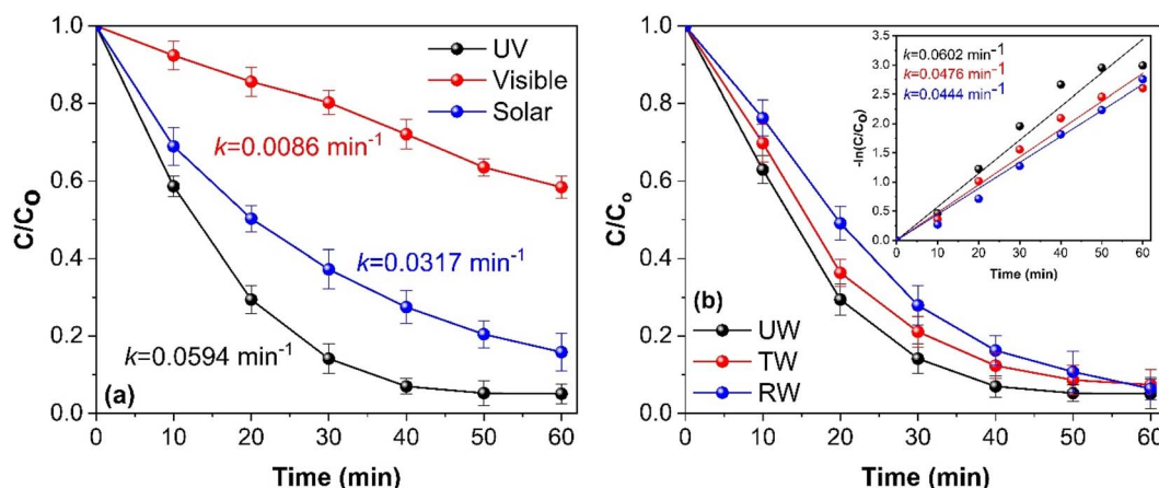
Fig. 6 (a) Effect of different light sources and (b) water matrix on the photocatalytic degradation of PCP (inset: rate kinetics). [(PCP) 0 = 10 \text{ mg L}^{-1} , CGBT dosage of 1 \text{ g L}^{-1} , pH 5, and UV light irradiation].
