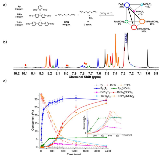
Fig. 9 (a) [3 \times 2] trigonal prismatic \text{DC}_{\text{ovL}} generated from 3\text{Py} + 3\text{BiPh} + 3\text{TriPh} + 2\text{T} + 6\text{NON} ; (b) partial ^1\text{H} NMR spectrum (400 MHz, \text{CDCl}_3 ) of the equilibrated reaction mixture; (c) ^1\text{H} NMR monitoring of macrocycles and macrocyclic cages over 2340 min. The initial concentration of each dialdehyde was 1.0 mM. Error in ^1\text{H} -NMR signal integration: \pm 5\% . The signals of free dialdehydes BiPh and TriPh are indicated by red and orange stars, respectively. The spectra and kinetic curves are coloured in accordance with the molecular structures.
