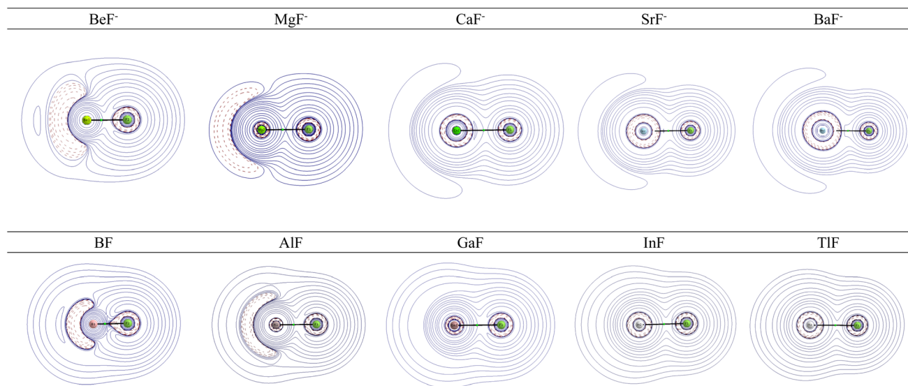
Fig. 2 Laplacian distribution \nabla^2\rho(r) of AeF - (Ae = Be–Ba) and EF (E = B–Tl) at the CCSD(T)/def2-TZVPP level. Red lines indicate the areas of charge concentration ( \nabla^2\rho(r) < 0 ), while blue lines show the areas of charge depletion ( \nabla^2\rho(r) > 0 ). The solid lines connecting the atomic nuclei are the bond paths. Green dots are bond critical points.
