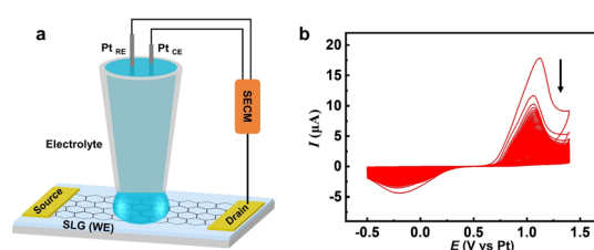
Fig. 1 (a) Schematic diagram of SLG bromination process. (b) Cyclic voltammograms of SLG microstrip electrode in an aqueous solution with 10 mM KBr and 10 mM H_2SO_4 ; the scan rate is 100 mV s^{-1} .
