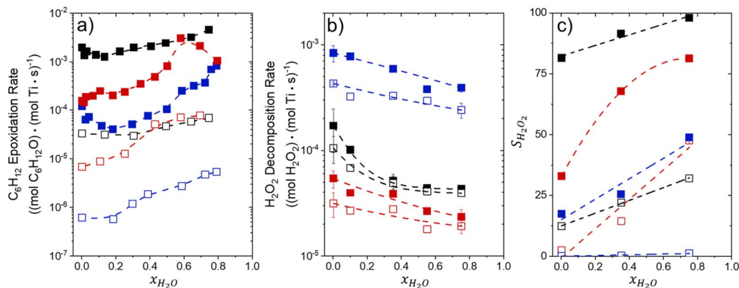
Fig. 1 Turnover rates for (a) C 6 H 12 epoxidation to form C 6 H 12 O (1 mM C 6 H 12 , 10 mM H 2 O 2 , 313 K), (b) H 2 O 2 decomposition (1 mM H 2 O 2 , 10 mM C 6 H 12 , 313 K) as a function of H 2 O mole fraction in mixtures of CH 3 CN (■, □), CH 3 OH (■, □), and C 4 H 6 O 2 (■, □) with H 2 O over Ti-BEA-OH (solid points) and Ti-BEA-F (hollow points). The furthest left data points represent x_{H_2O} = 0.002 , which comes from the aqueous H 2 O 2 reagent solution (39 mM).
