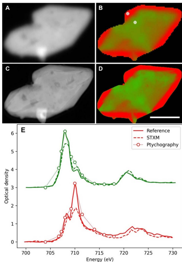
Fig. 13 Comparison between conventional STXM (A and B) and ptychographic (C and D) spectromicroscopy images of Li x FePO 4 micro-platelets. The average optical density (A and C) and the chemical composition map (B and D) where the two chemical components (LiFePO 4 and FePO 4 ) are presented in green and red, respectively (scale bar is 1 μm; reconstructed pixel size 5 nm). (E) Point spectra from the dots marked in (B) by conventional STXM (dashed lines) and ptychographic modes (dotted lines with circles). Reference spectra from pure materials (LiFePO 4 , green solid line; FePO 4 , red solid line) are also shown for comparison. The conventional STXM spectra show distortions that flatten the sharpest peaks, corresponding to energies where the difference in absorption between phases is maximum. The different attenuation overweighs the more abundant phase and instead the ptychographic spectra more closely match the pure references. Reproduced from ref. 157.
