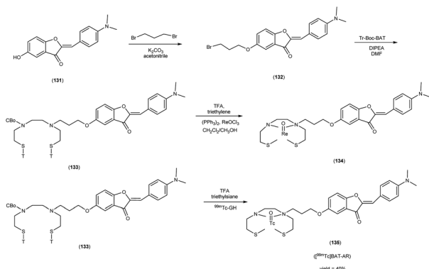
Scheme 11
