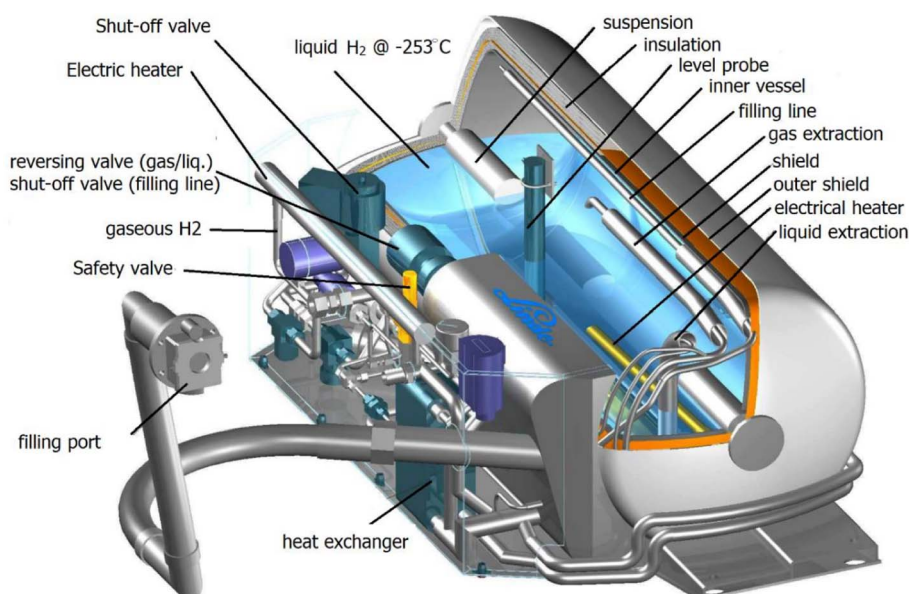
Fig. 20 Schematic of a cryogenic hydrogen tank. 133 Reproduced from ref. 133 with permission from [MDPI], copyright [2020].
