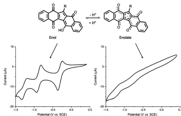
Fig. 5 Cyclic voltammetry of KuQEt in CH_2Cl_2 /TBAP 0.1 M (left) and DMF/TBAP 0.1 M (right). WE: glassy carbon, RE: saturated calomel electrode, CE: platinum wire. Adapted from ref. 29. Copyright 2021 The Authors. Published by American Chemical Society.
