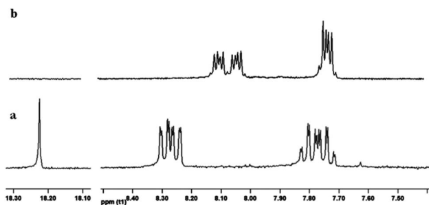
Fig. 4 Comparison between ^1H -NMR spectra of KuQTEGMe in (a) CDCl_3 , (b) DMSO-d_6 . Reprinted with permission from ref. 27. Copyright 2017 American Chemical Society.
