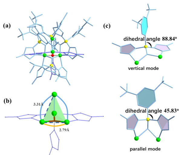
Fig. 3 (a) Molecular structures of AlOC-127 and the coordination environment of \text{Al(III)} ; (b) core structure of AlOC-127 . The vertical mode and parallel mode of \text{L}^2 ligands are presented as blue and yellow lines for clarity. (c) The presentation of the vertical mode and parallel mode of \text{L}^2 ligands (color code: Al, green; B, yellow; O, red; N, blue; C, black).
