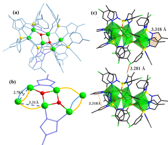
Fig. 4 (a) Molecular structures of AlOC-128 and the coordination environment of \text{Al(III)} and (b) the core structure of AlOC-128 . The vertical mode and parallel mode of \text{L}^2 ligands are presented as blue and yellow lines for clarity. (c) The intramolecular and intermolecular interactions (color code: Al, green; B, yellow; O, red; N, blue; C, black).
