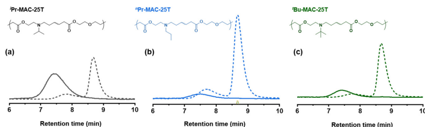
Fig. 4 SEC analysis of copolymers before (solid lines) and after hydrolytic degradation (dashed lines) under accelerated conditions. Light scattering signals of (a) 1 Pr-MAC-25T, (b) 1 Pr-MAC-25T and (c) t Bu-MAC-25T are depicted.
