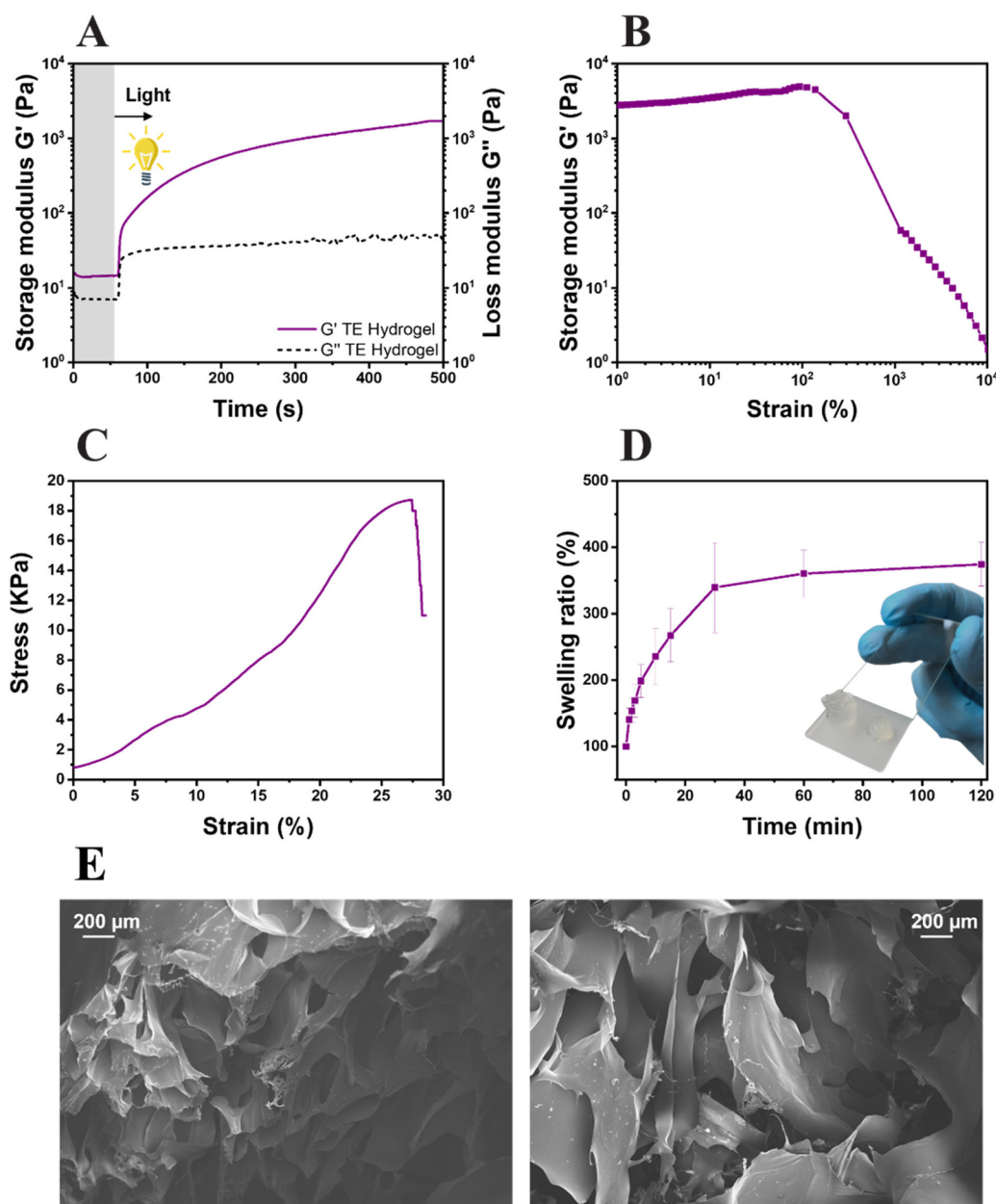
Fig. 4 Potorheology (A), amplitude sweep (B), compression test (C) and swelling kinetics (D) of the thiol-ene hydrogel (TE hydrogel). Field Emission Scanning Electron Microscopy (FESEM) of the TE hydrogels; scale bar 200 \mu\text{m} (E).
