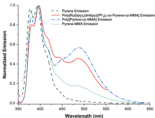
Fig. 5 Normalized emission spectra of pyrene species used in this study in DMSO; excitation wavelength = 335 nm. The pyrene excimer emission is observed centered at ~488 nm.
