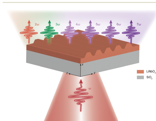
Fig. 1 Schematic of HHG from a \text{LiNbO}_3 metasurface supporting guided-mode resonance. When the TE-polarized pump laser is normally incident from the substrate side, the nonlinear harmonic signals from the 2 nd to 7 th order are emitted in the transmission direction. The metasurface is composed of a \text{LiNbO}_3 grating whose optical axis is along the z -direction situated on a \text{SiO}_2 /quartz substrate.
