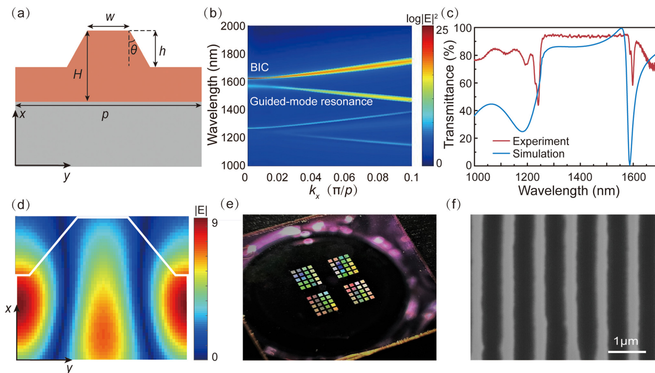
Fig. 2 (a) Schematic illustration of a unit cell of the \text{LiNbO}_3 metasurface. The geometric parameters are w = 260 \text{ nm} , h = 240 \text{ nm} , H = 600 \text{ nm} , p = 850 \text{ nm} , and \theta = 45^\circ . (b) Calculated band structure of the \text{LiNbO}_3 metasurface. (c) Measured (red) and simulated (blue) transmittance spectra of the \text{LiNbO}_3 metasurface, respectively. (d) Simulated electric field distribution in the x - y plane at a resonant wavelength of 1580 \text{ nm} . The box illustrates the \text{LiNbO}_3 region. (e) An optical photo of the fabricated \text{LiNbO}_3 metasurface. (f) A representative SEM image of the fabricated \text{LiNbO}_3 metasurface.
